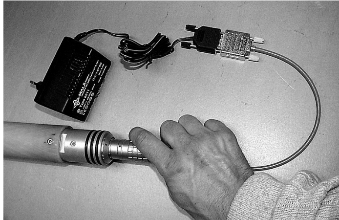
Figure 5.11. Connecting the battery charging to Rx antenna.
