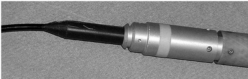
Figure 4.3. Optical cable-head connected to probe.
