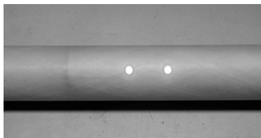
Figure 6.2. Diode on the 100 MHz Rx antenna
