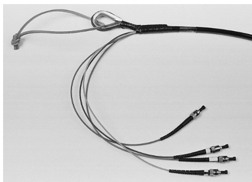
Figure 2.1. Optical cable termination and strain relief.
