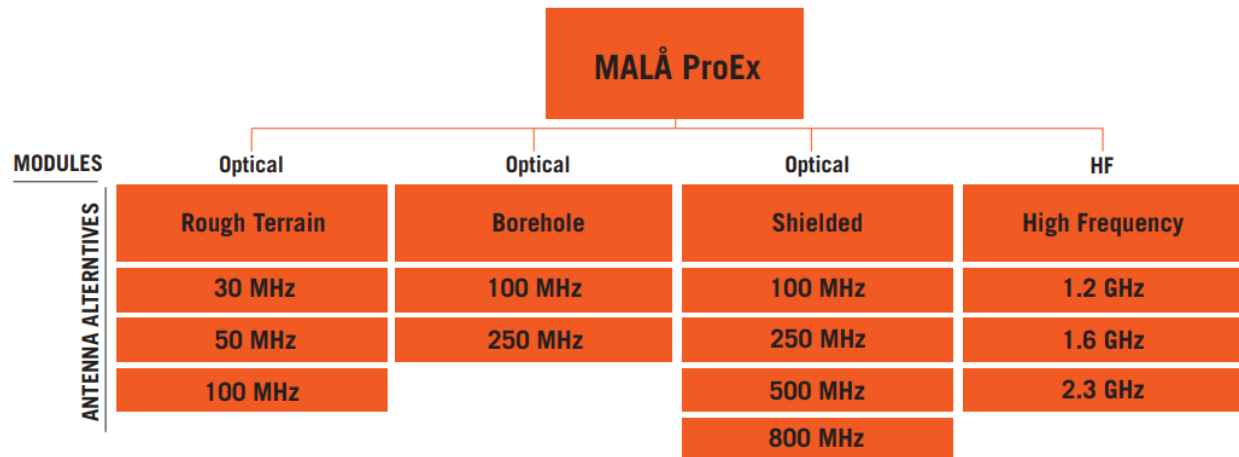
Figure 2.1 An overview of all antennas that can be used together with the ProEx. For latest update, visit Guideline Geo's homepage, www.guidelinegeo.com
