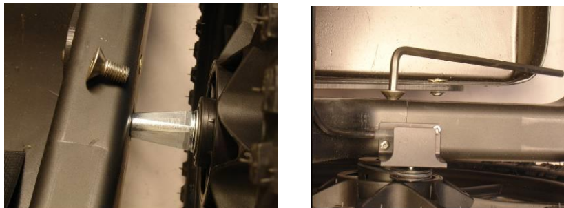
Figure 7.8 Attachment of wheel.
