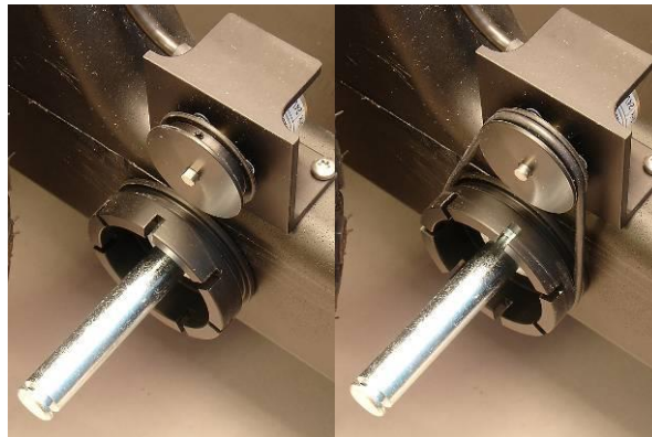
Figure 7.7 The O-ring attached to the wheel axles.
