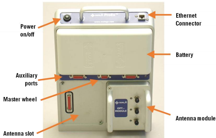
Figure 2.2 The MALÅ ProEx Control unit.
