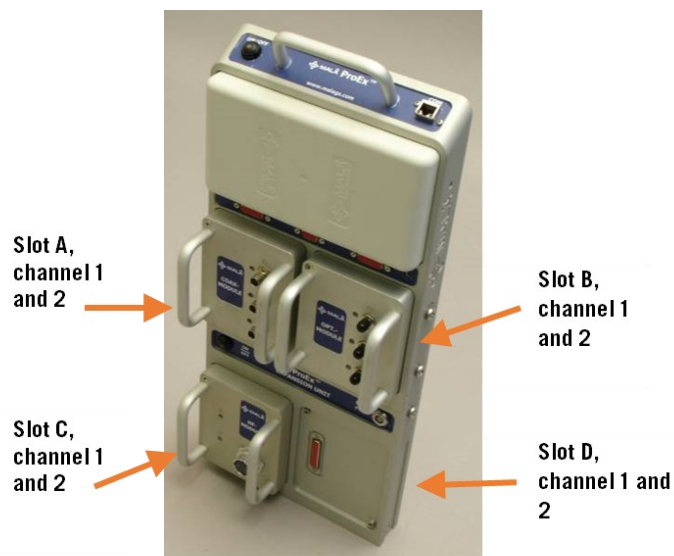
Figure 10.2 The ProEx with one expansion unit and three antenna modules. To this set up two more expansion units can be connected.
